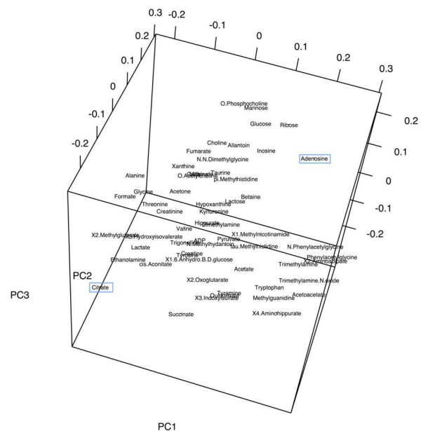
Figure 3. Principal component (PC) loadings plot of urinary metabolic profiles shows the influence of the metabolites on the scores. It can be seen that citrate and adenosine (boxed) are well-separated in the model.
