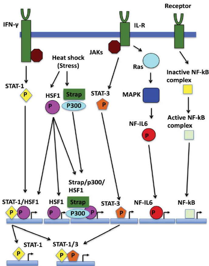
Figure 2 Signal pathway integration that regulates Hsp90 expression. Known signaling pathways that affect expression of Hsp90 and various scenarios for binding. Not shown is the co-activator Daxx, which is known to promote HSF1 activation. [83]. The blue rectangles represent the Hsp90 promoter regions upon which various combinations of transcription factors operate. STAT1 may function independently of HSF1 or with STAT3. IFN- \gamma , interferon- \gamma ; IL-R, interleukin receptor; JAK, Janus kinase; MAPK, mitogen-activated protein kinase.
