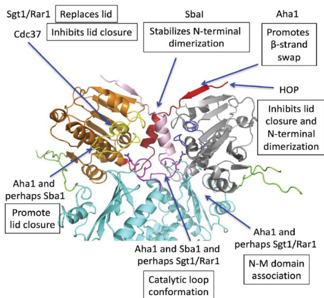
Figure 3 Points of co-chaperone action on structural elements of Hsp90 essential for its ATPase activity. Cdc37 p50 prevents molecular rearrangement of the lids of Hsp90. HOP may prevent lid closure and N-terminal dimerization probably by interacting with the N-terminal segments of Hsp90. Aha1 appears to interact with all the structural elements leading to a co-operative N-terminally dimerized state of Hsp90. Sba1 can stabilize Hsp90 complexes by reducing the ATPase activity of Hsp90 and it appears to interact with both the lid and N-terminal domains of Hsp90. Sba1 may also modulate the middle domain catalytic loop. Sgt1-Rar1 complex, appear to activate Hsp90 in an open state and convert it to a stable ADP-bound state.
