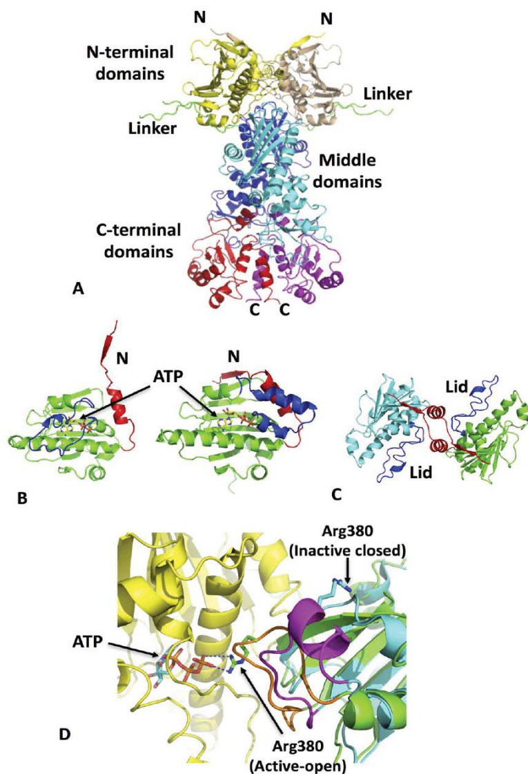
Figure 1 The structure and conformational changes of the Hsp90 chaperone. (A) The closed conformation of the Hsp90 dimer showing transient N-terminal domain (yellow and brown) dimerization. Middle domains are colored blue and cyan while C-terminal domains are shown in red and magenta. The charged linker is shown in green. (B) Conformation of the lid and N-terminal segment of the Hsp90 N-terminal domains. The closed undimerized state is shown in the left-hand panel and the open dimerized state in the right-hand panel. Lids are colored in blue and N-terminal segment in red. (C) The N-terminally dimerized state of Hsp90 (cyan and green). Lids are shown in blue and N-terminal segment in red. N-terminal dimerization involves a series of cooperative structural movements including the N-terminal and lid segments. (D), Catalytic loop conformation of Hsp90. Hsp90 N-terminal domain is shown in yellow. Two superimposed Hsp90 molecules (cyan and green) represent the middle domain. The closed inactive catalytic loop is shown in magenta and the open active state in orange and interacting with bound ATP (stick model). Arg380 of the catalytic loop interacts with ATP only in the active state (or open state). Hydrogen bonds are represented by broken blue lines.
