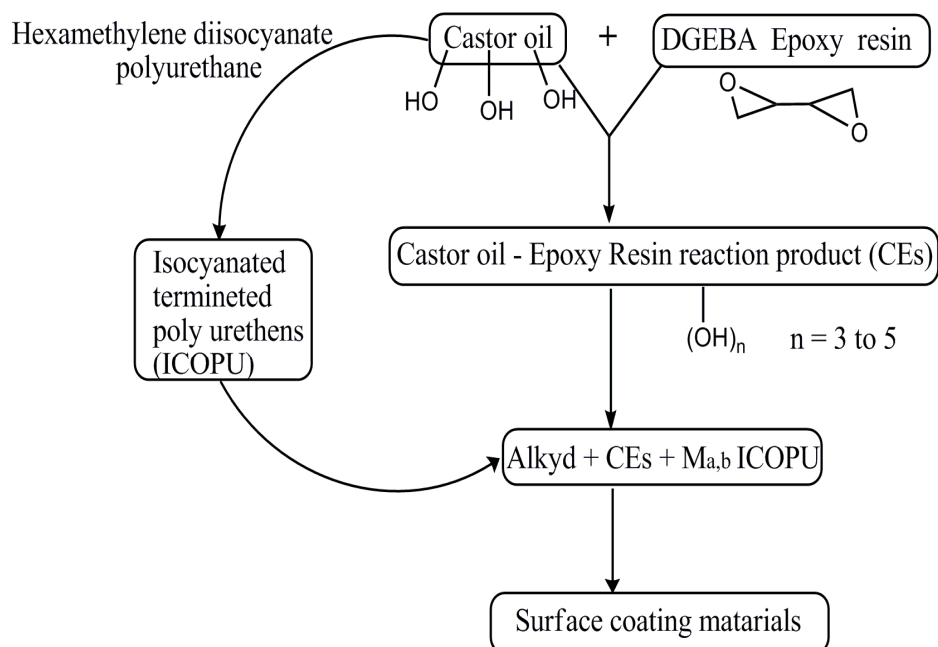
Scheme 1. Surface coating materials based on blending of alkyd resin, CE and ICOPU
