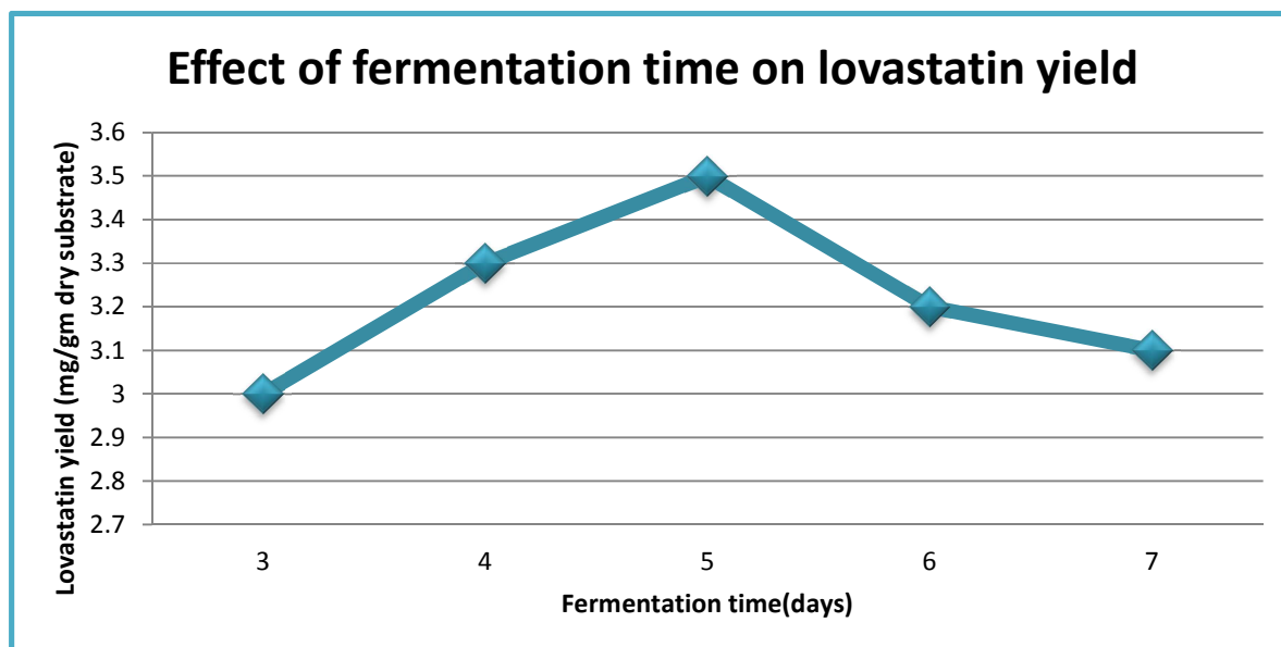
Fig. 2: Effect of fermentation time on lovastatin production
