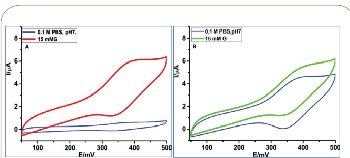
Figure 4 Cyclic voltammograms of (A) PVP-Os/chitosan/ rGcGDH , and (B) PVP-Os/ rGcGDH , at scan rate 5 \text{mV/s} , in 0.1 M PBS pH 7.4 and in 15 mM glucose vs. \text{Ag}|\text{AgCl} (KCl sat.).
