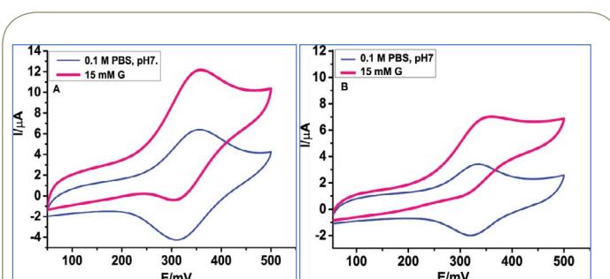
Figure 2 Cyclic voltammograms of (A) PVP-Os/chitosan/ fdgAmPDH , and (B) PVP-Os/ fdgAmPDH in 0.1 M PBS pH 7.4 and in 15 mM glucose vs. \text{Ag}|\text{AgCl} (KCl sat.), and a 5 \text{mV/s} scan rate.
