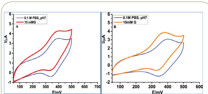
Figure 3 Cyclic voltammograms of (A) PVP-Os/chitosan/ gAmPDH , and (B) PVP-Os/ gAmPDH , at scan rate 5 \text{mV/s} and 15 mM glucose in 0.1 M PBS pH 7.4 vs. \text{Ag}|\text{AgCl} (KCl sat.).
