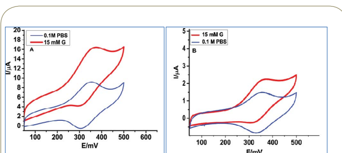
Figure 1 Cyclic voltammograms of (A) PVP-Os/chitosan/ AnGOx and (B) PVP-Os/ AnGOx , in 0.1 M PBS pH 7.4 (blue color) and in 15 mM glucose (red color), vs. \text{Ag}|\text{AgCl} (KCl sat.) 5 \text{mV/s} scan rate.
