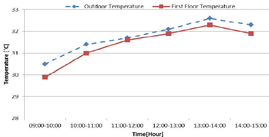
Fig 6 First floor space (2A) as related to outdoor in terms of temperature
