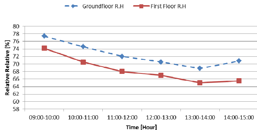
Fig 12 Ground floor as related to first floor in terms of relative humidity (R.H.)
