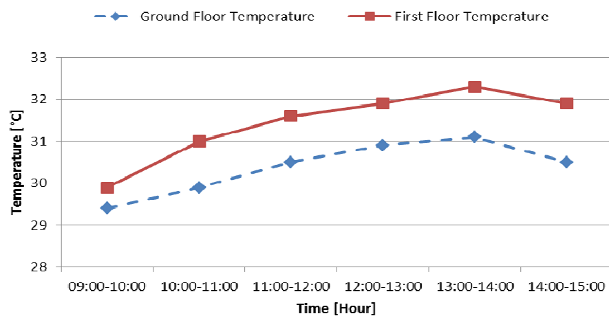
Fig 7 Ground floor as related to first floor in terms of temperature
