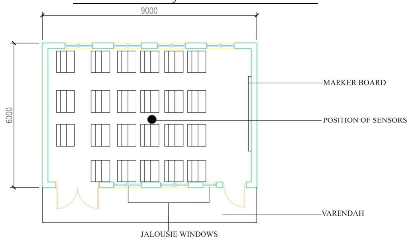
Fig 3 Location of sensors in the classrooms
