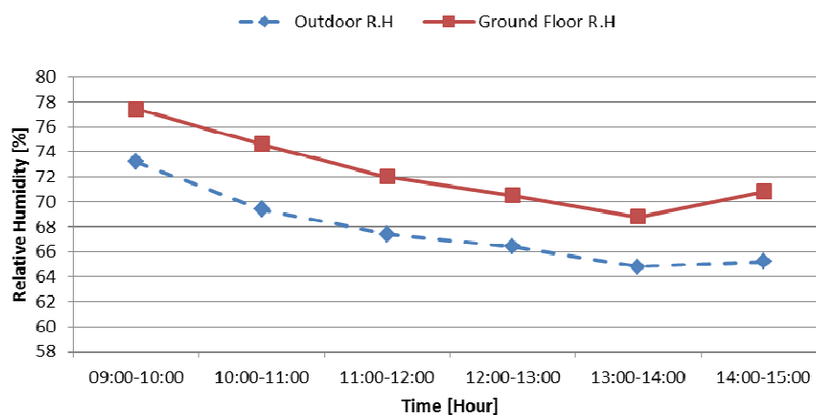
Fig 11 Ground floor as related to outdoor in terms of relative humidity
