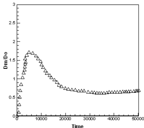
Fig. 7. A results for the evolution of nondimensional maximum lateral spread ratio of 6 nm diameter nanodroplet impacting on partially wettable surface. for a case with V_0 = 1.25\text{ms}^{-1} .
