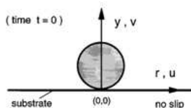
Fig. 1. A schematic of a droplet impact on a surface.
