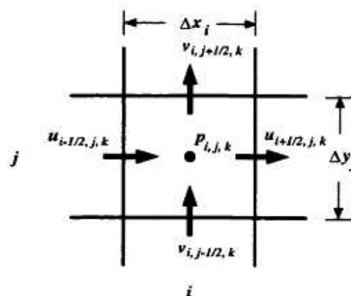
Fig. 2. A 2D control volume, with velocities specified at cell faces, pressure at the cell center.
