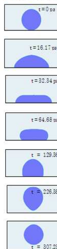
Fig. 5. CFD-MK images of a 6 nm nanodroplet impacting with a velocity of 1.25 m/s on flate non-wettable surface.
