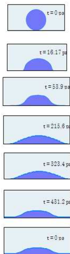
Fig. 3. CFD-MK images of a 6 nm nanodroplet impacting with a velocity of 1.25 m/s on flate wettable surface.
