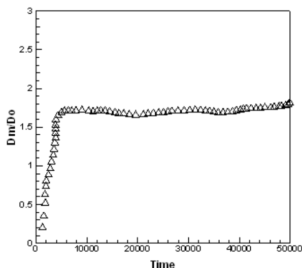
Fig. 6. A result for the evolution of no dimensional maximum lateral spread ratio of 6 nm diameter nanodroplet impacting on wettable surface. for a case with V_0 = 1.25\text{ms}^{-1} .
